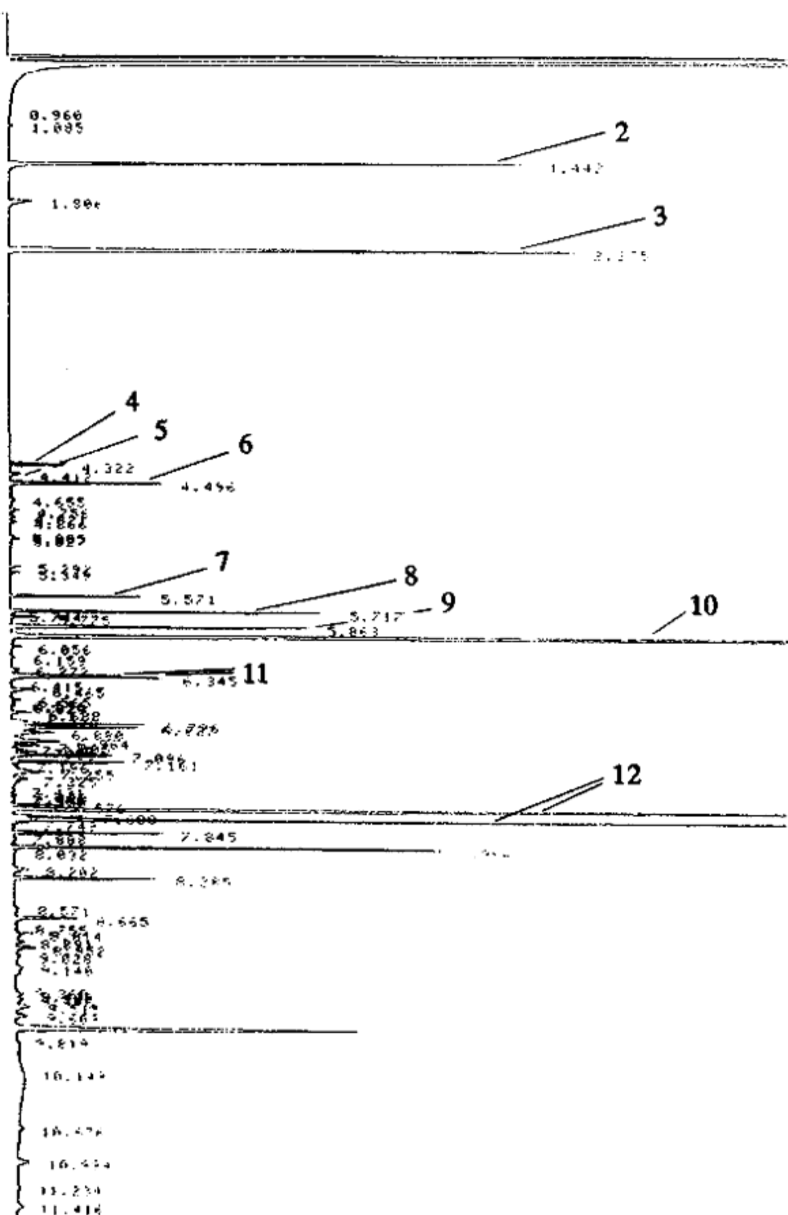
FIG. 1—Gas chromatogram of Mixture A, an oily liquid seized from an illicit laboratory. See Experimental section for chromatographic conditions.
